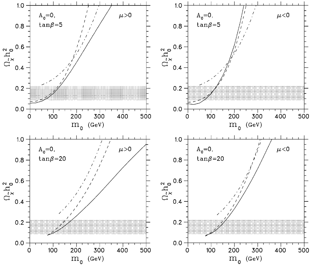
FIG. 2. The relic density as function of m_0 for fixed values of the remaining parameters. The solid, dashed and dot-dashed lines correspond to M_{1/2}=170, 200, \text{ and } 400 GeV, respectively.
