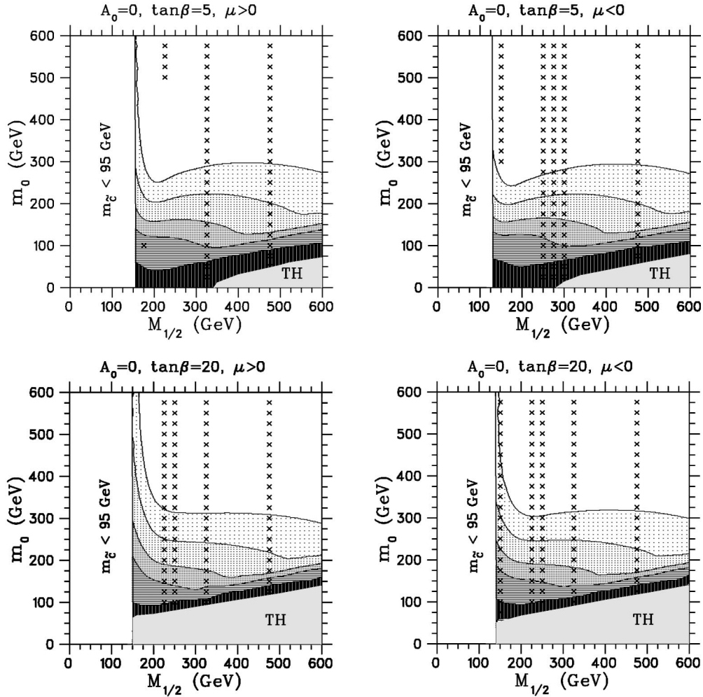
FIG. 10. The LSP relic density \Omega_{\tilde{\chi}_0} h_0^2 in the (m_0, M_{1/2}) plane for given values of A_0 , \tan \beta , and sign of \mu when coannihilation effects are taken into account. The inputs are the same as in Fig. 1.
