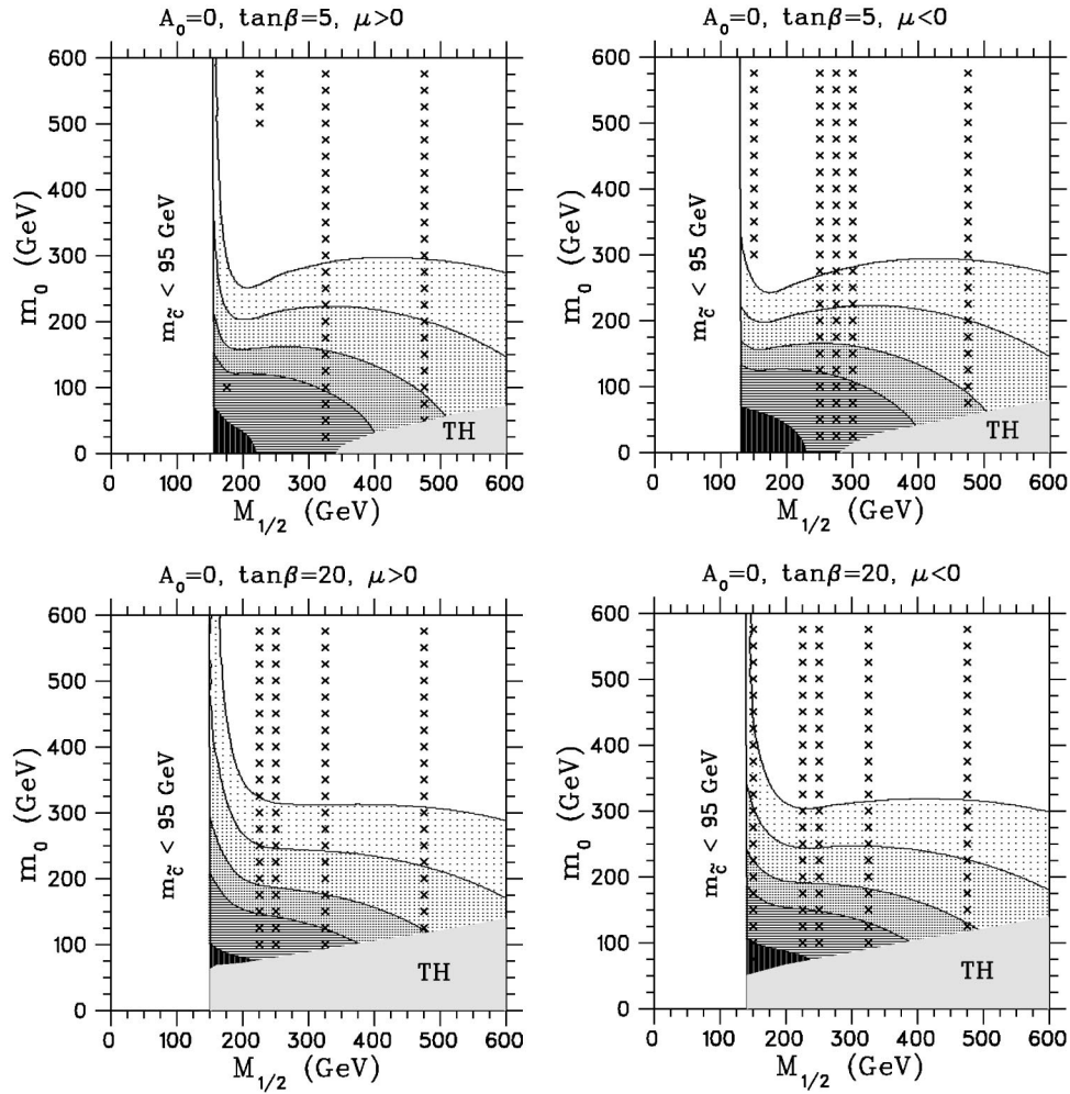
FIG. 1. The LSP relic density \Omega_{\tilde{\chi}h_0^2} in the (m_0, M_{1/2}) plane for given values of A_0, \tan\beta , and sign of \mu . Gray tone regions, from darker to lighter, designate areas in which the LSP relic density takes values in the intervals 0.00–0.08, 0.08–0.22, 0.22–0.35, 0.35–0.60, and 0.60–1.00, respectively. In the blanc area \Omega_{\tilde{\chi}h_0^2} > 1.0 . The area marked by TH is theoretically excluded (see main text). The area labeled by m_{\tilde{\chi}} < 95 GeV is excluded by chargino searches. Crosses denote points for which thresholds or poles are encountered.
